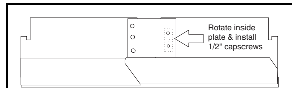
Figure 3 - 36 5/8" Cap Screws - Location
