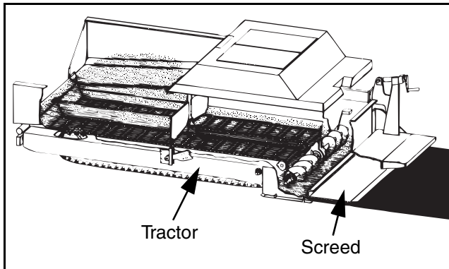
Figure 3 - 1 Asphalt Flow
