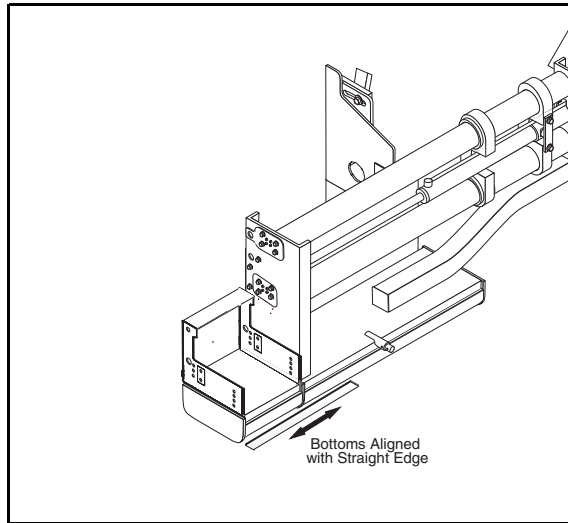
Figure 3 - 30 Checking Parallel Alignment
