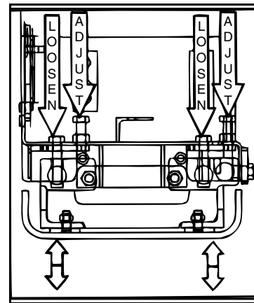
Figure 3 - 33 Adjustment Screw Locations
