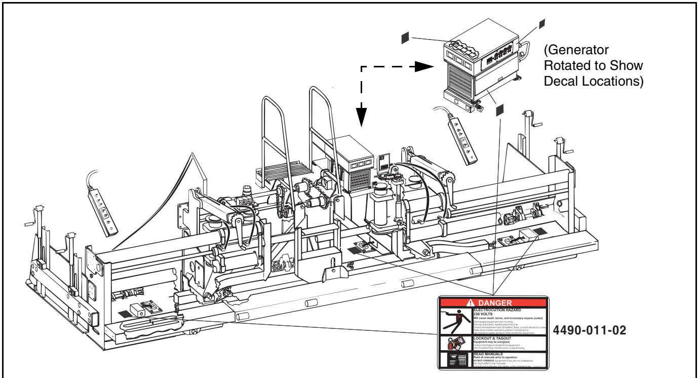
Figure 2 - 7 Additional DANGER! Decal Locations Found on Stretch 18 Models with Electric Screed
