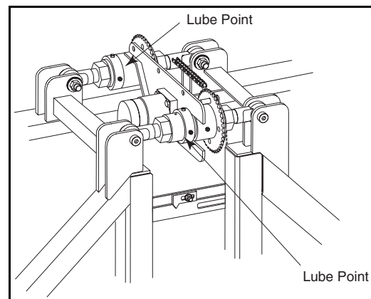
Figure 3 - 42 Crown Lubrication Points
