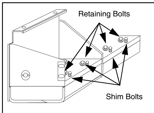
Figure 3 - 20 Adjusting Angle of Attack
