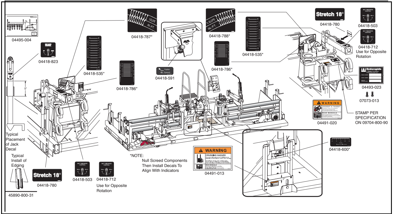
Figure 2 - 6 Decal Locations on Stretch 18 - All Models
