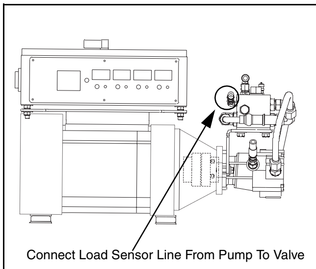
Figure 5 - 5 Tractor Generator Pump Connection on Screed Generator Drive Motor
