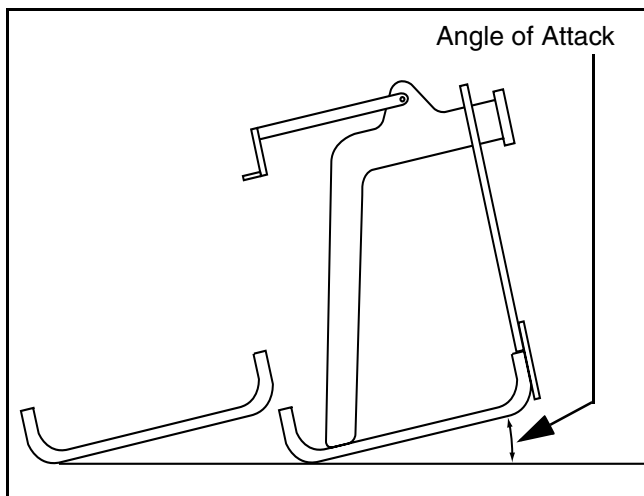
Figure 3 - 6 Screed Angle of Attack
