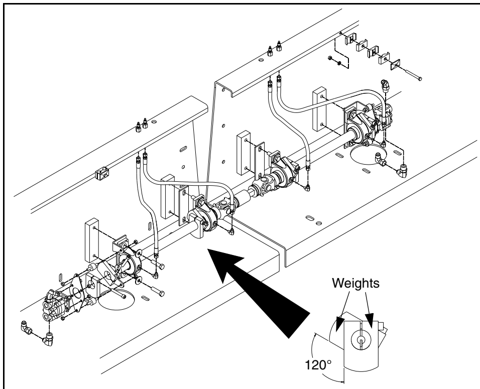
Figure 3 - 25 Vibrator Weight Eccentric Installation & Alignment
