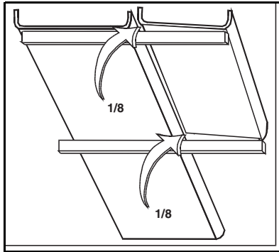
Figure 3 - 19 Gap Between Edges
