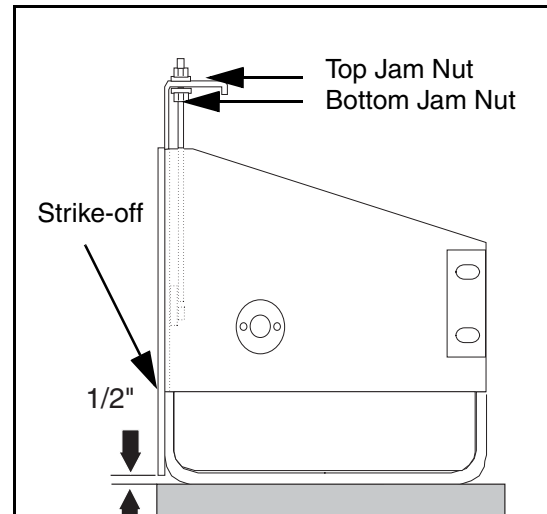
Figure 3 - 26 Strike-Off Adjustment
