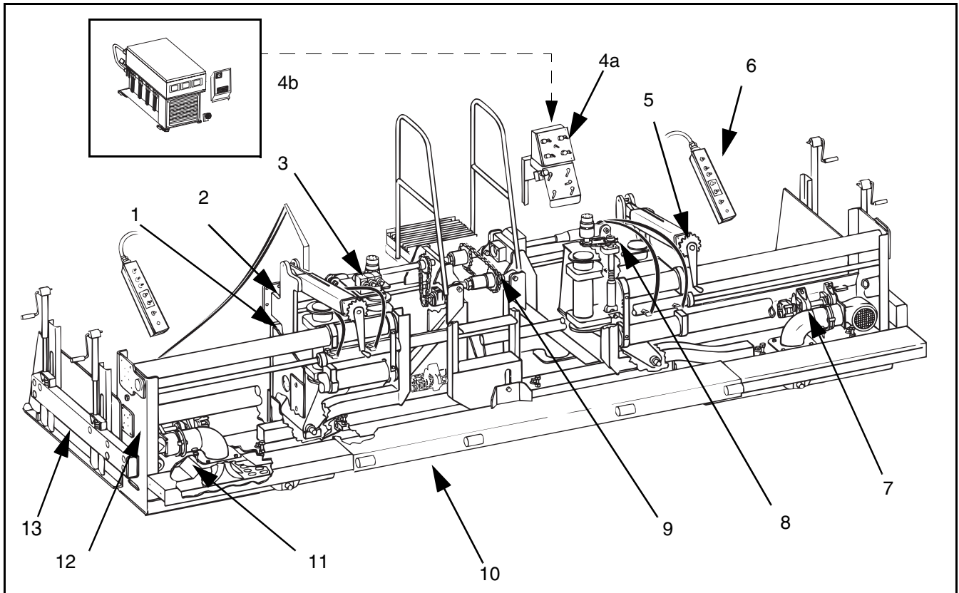
Figure 3 - 2 Stretch 16 & 18 Screed Components
