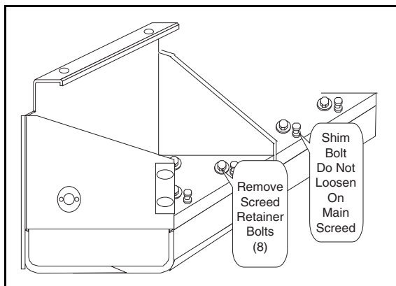
Figure 3 - 37 5/8" Shim Bolt Location
