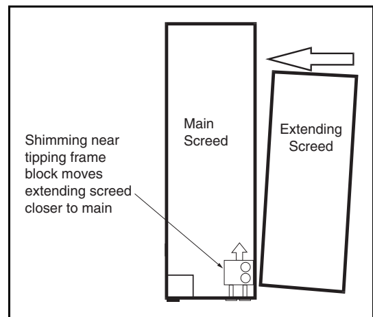
Figure 3 - 21 Extending Screed Alignment
