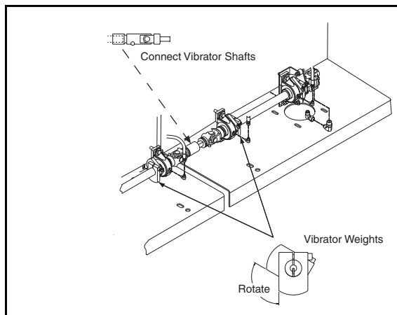
Figure 3 - 28 Vibrator Shaft Alignment
