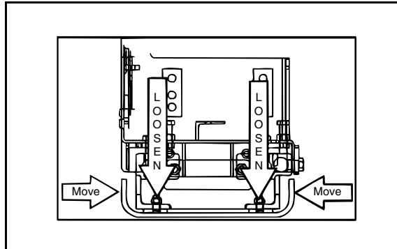
Figure 3 - 31 Aligning Extension Bottom
