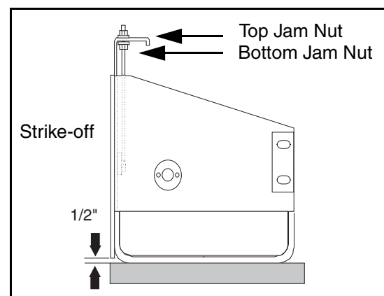
Figure 3 - 17 Strike-Off Adjustment
