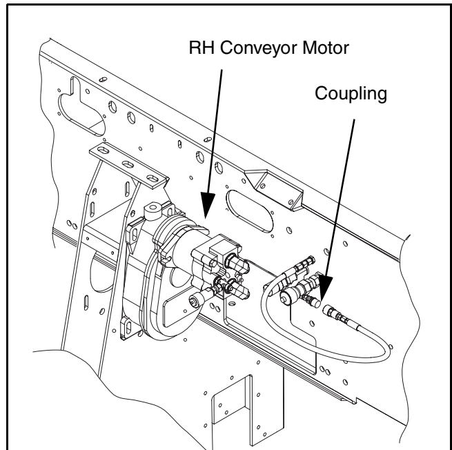
Figure 5 - 6 Generator Pump Connections for Detached Screed
