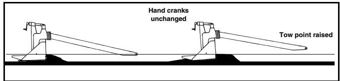
Figure 13 Angle Change Moving Tow Point
