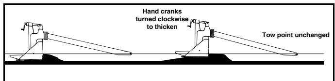
Figure 14 Angle Change Moving Hand Crank
