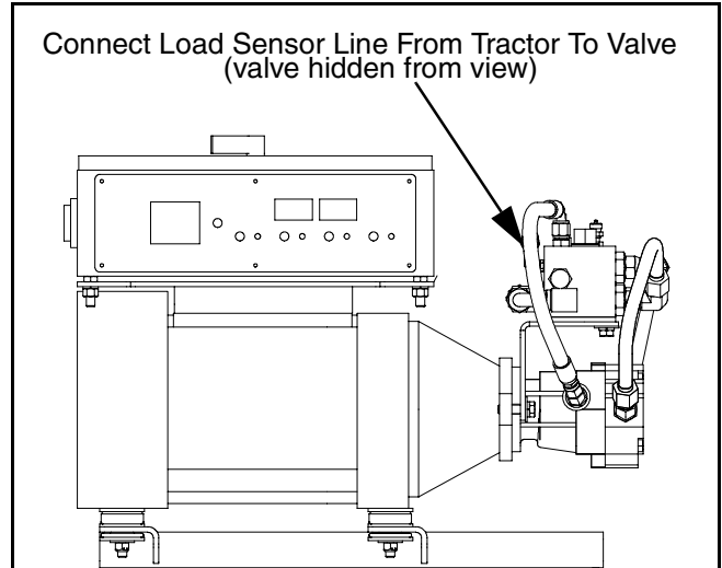
Figure 35 Tractor Generator Pump Connection on 8-Foot Screed Generator Drive Motor
