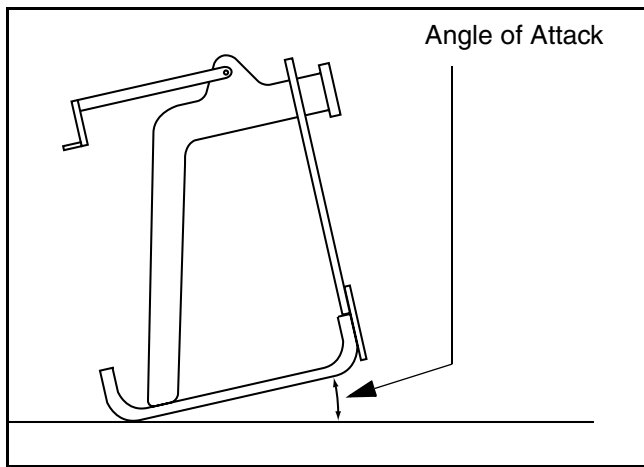
Figure 12 Screed Angle of Attack
