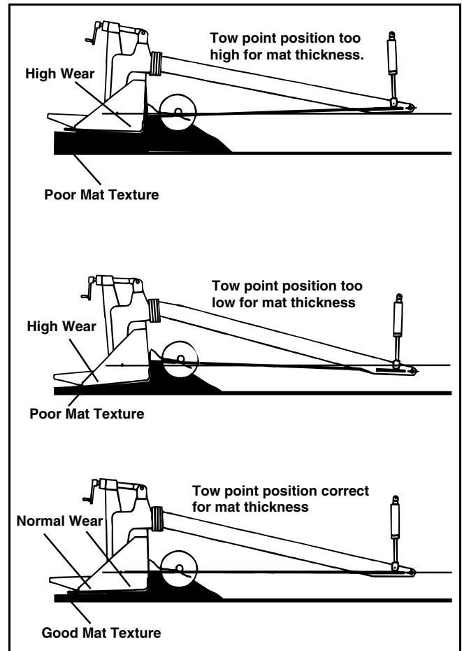
Figure 18 Effects of Tow Point Position
