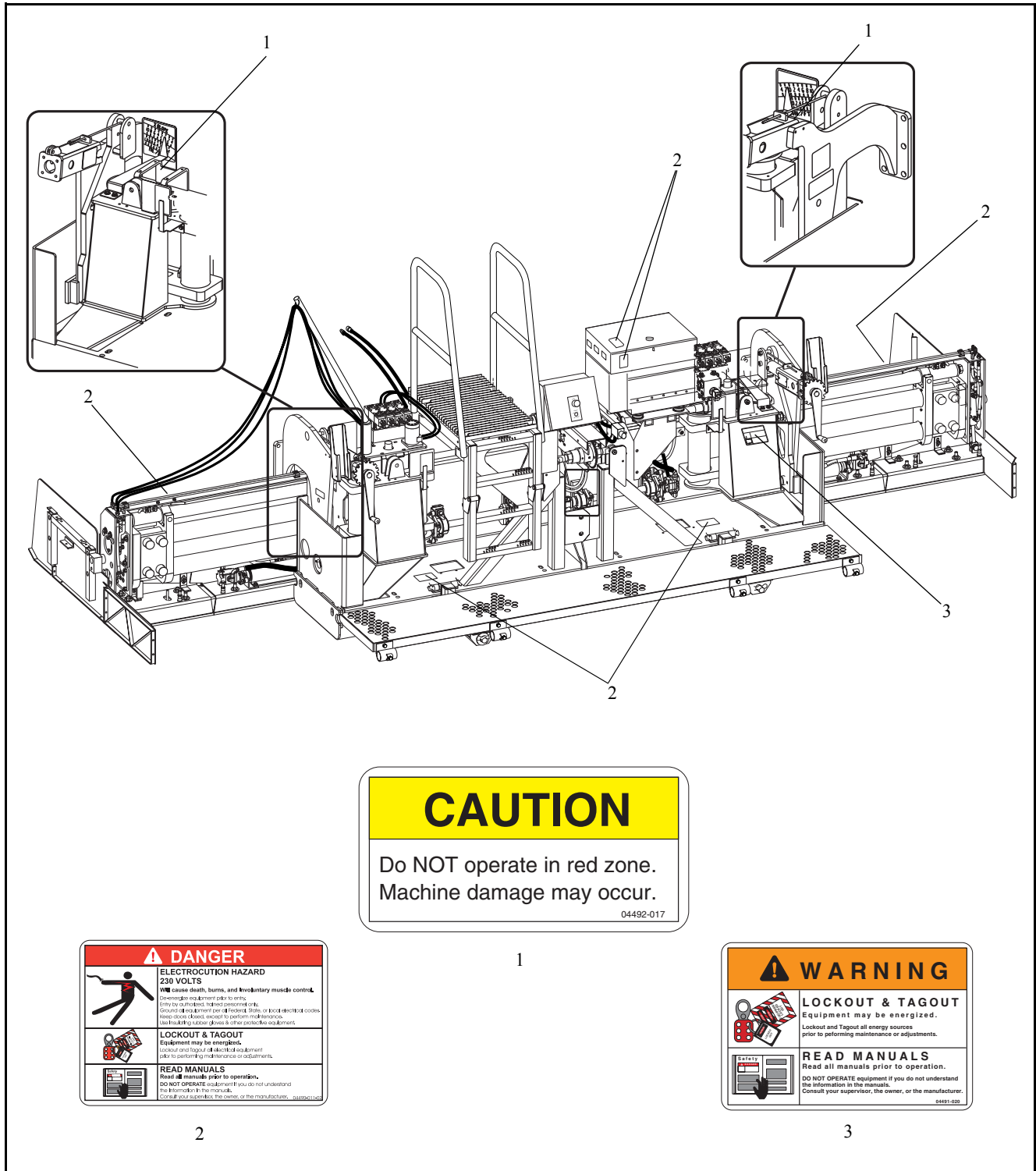
Figure 4 Safety Decal Location
