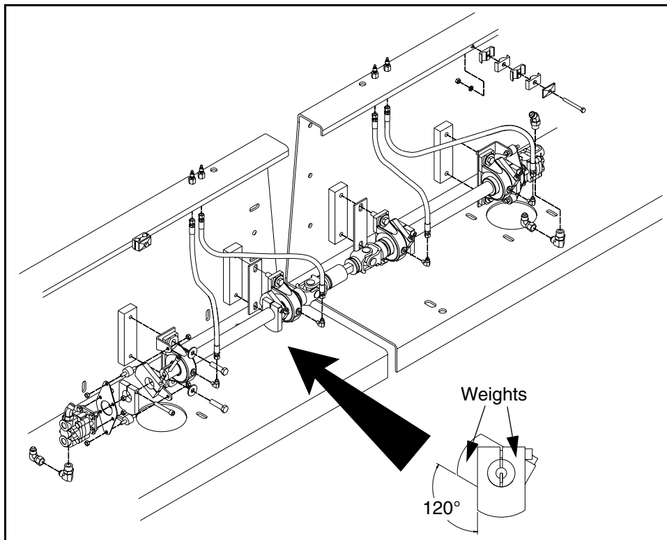
Figure 26 Vibrator Weight Installation & Alignment
