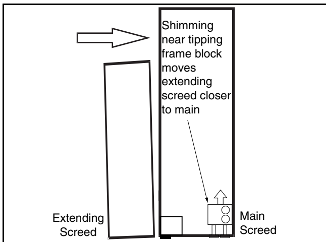
Figure 24 Extending Screed Alignment
