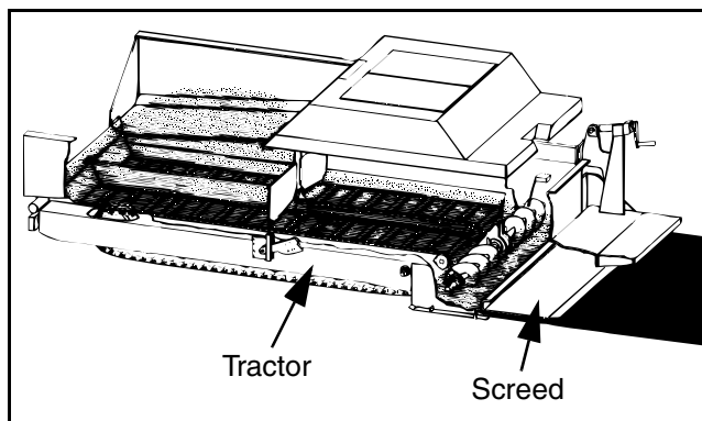
Figure 5 Asphalt Flow
