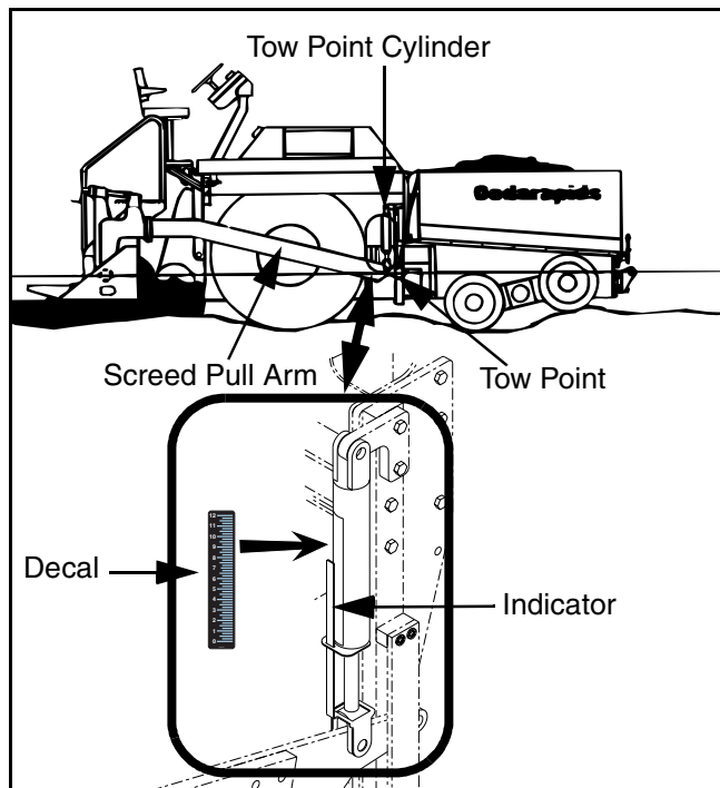
Figure 17 Tow Point Indicator
