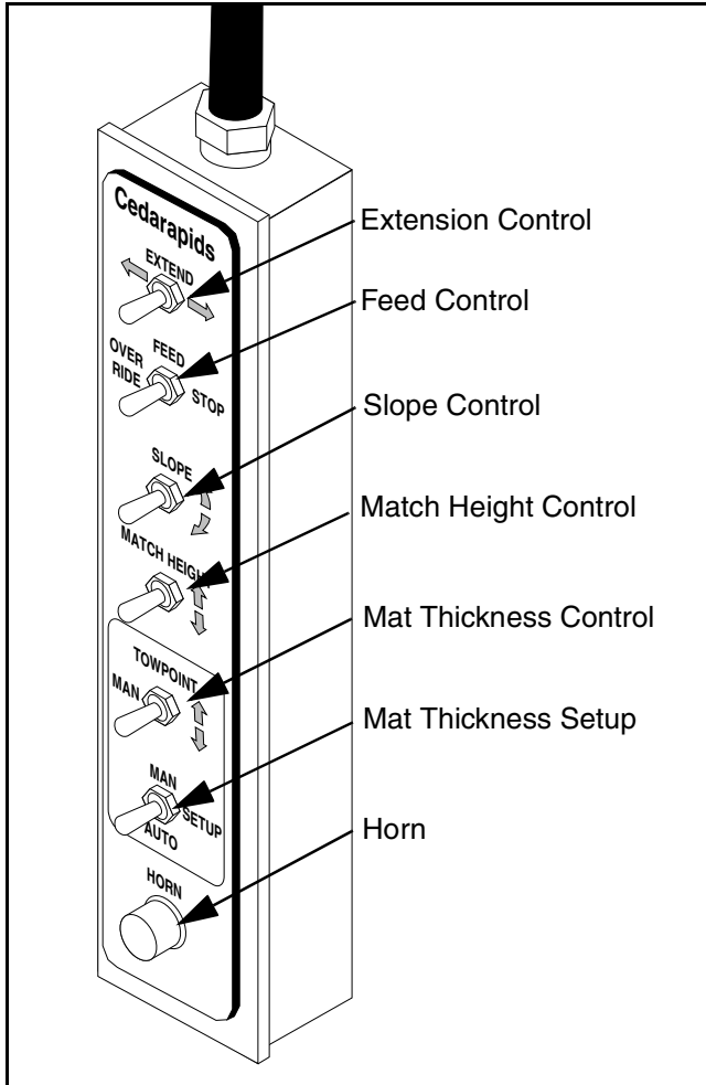
Figure 9 Remote Control Panel
