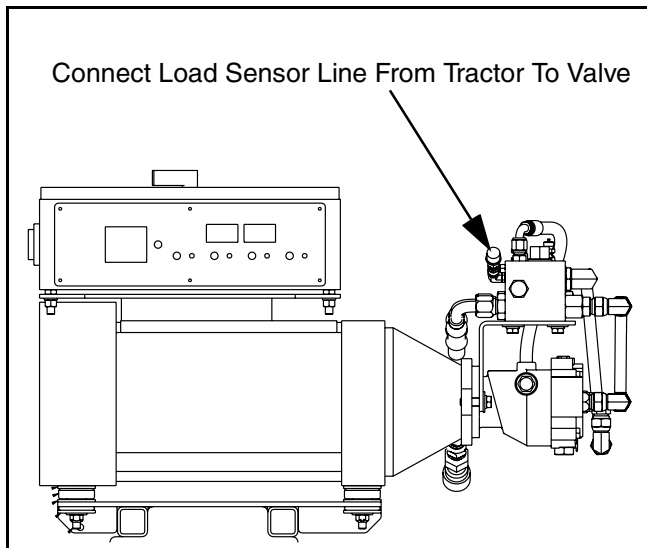
Figure 34 Tractor Generator Pump Connection on 10-Foot Screed Generator Drive Motor
