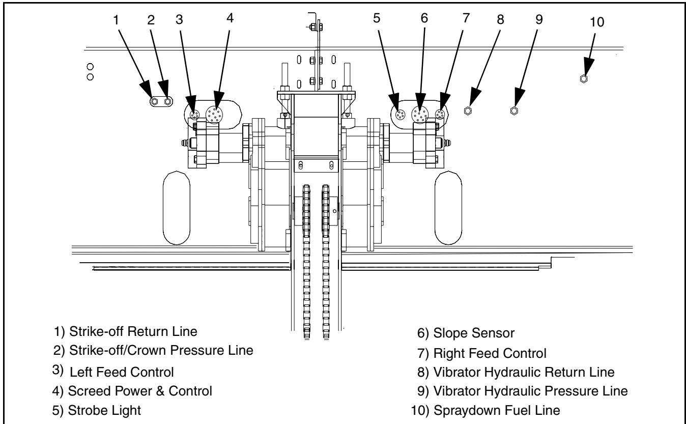
Figure 11 Hydraulic and Electrical Disconnects
