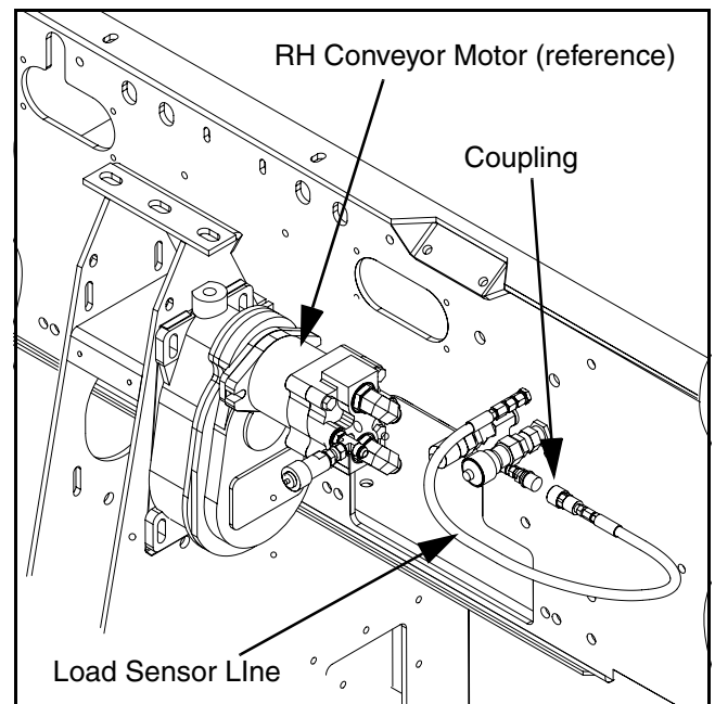
Figure 36 Generator Pump Connections for Detached Screed
